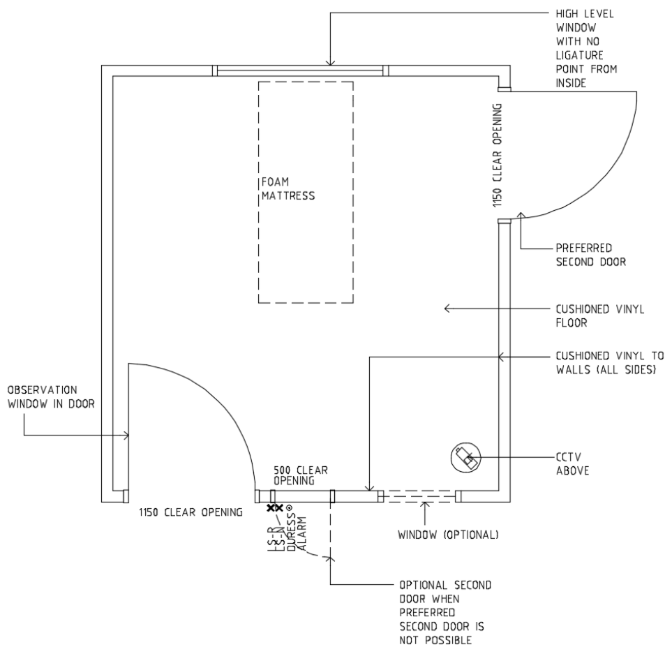
Figure 6.4: Recommended door openings for Seclusion Room
